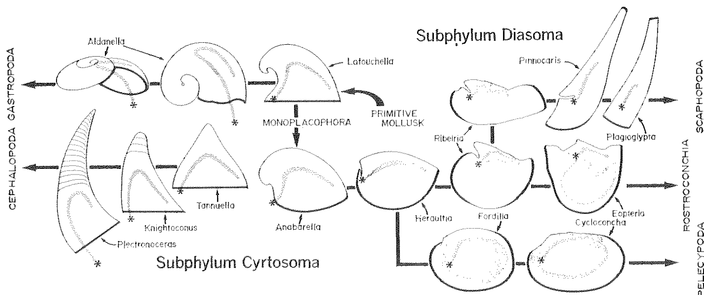
Fig. 4. Schematic view of the origin of the univalved and bivalved molluscan classes. Most drawings are based on internal molds of the shells. Thick lines show extent of shell apertures; stippled areas represent muscle insertions; shaded areas show probable position of gut with mouth indicated by asterisk.
