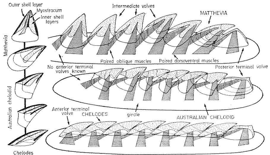
Fig. 5. Reconstructions of primitive Cambrian and Early Ordovician chitons known only from disarticulated plates.
