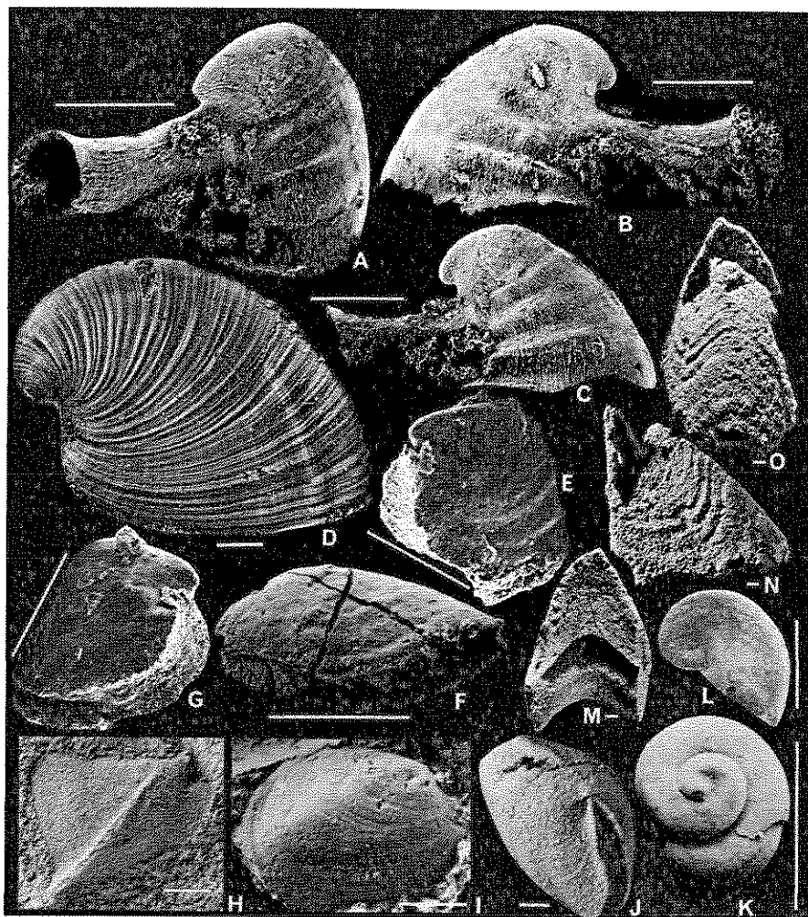
Fig. 3. Cambrian (A to L) and Early Ordovician (M to O) mollusks. (A to C) Yocheilcionella , Australian Cambrian monoplacophoran with anterior tube; (D) Anabarella , laterally compressed monoplacophoran, basal Cambrian, Siberia; (E to G) Heraltia , oldest known rostroconch, Early Cambrian, France; (H) Opikella , oldest known technophorid rostroconch, Late Cambrian, Australia; (I) Fordilla , oldest known pelecypod, Early Cambrian, United States; (J) Ribeiria , descendent of Heraltia , Late Cambrian, Australia; (K) Aldanella , oldest known gastropod, basal Cambrian, Siberia; (L) Pelagiella , gastropod, Early Cambrian, Great Britain; (M to O) ventral, right lateral, and dorsal views of intermediate valve of chelodid chiton, Early Ordovician, Australia. Bars equal 1 millimeter.
