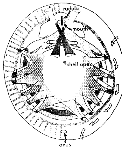
Fig. 2. Reconstruction of Rasetti's Middle Cambrian monoplacophoran Scenella , modeled from Neopilina . Stippled ring represents incipient pallial line indicated by change in slope of shell. Radial fluting of shell outside pallial line reflects weak radial mantle muscles (shown on left side only by short stippled lines). Also shown are radial and circular muscles of the foot as well as muscles controlling the head (anterior pair hypothetical). Arrows indicate probable direction of water flow through the mantle cavity.
